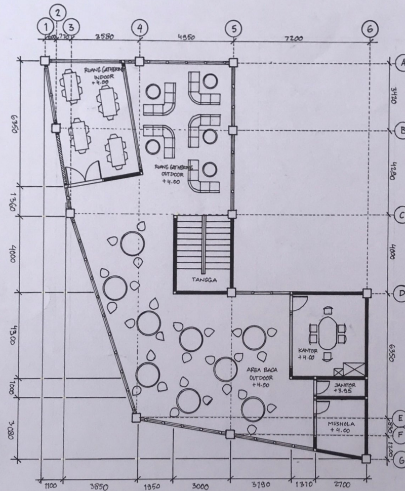
DENAH MICROLIBRARY LT.2 SKALA 1:100
